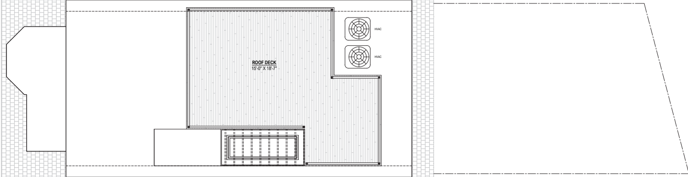
02 | PROPOSED ROOF DECK PLAN 3/16" = 1'-0"
