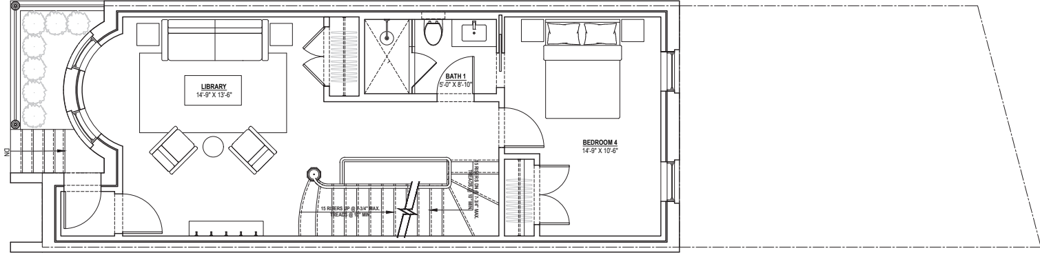
02 | PROPOSED STREET LEVEL PLAN 3/16" = 1'-0"
