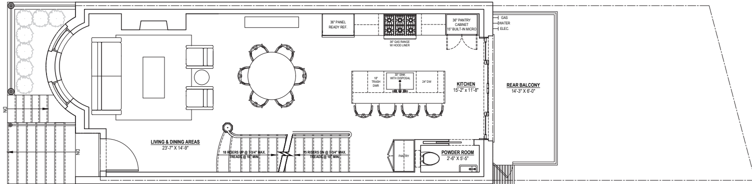
01 | PROPOSED PARLOR LEVEL PLAN 3/16" = 1'-0"
