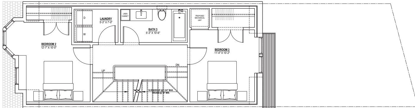
01 | PROPOSED SECONDARY BEDROOM LEVEL PLAN 3/16" = 1'-0"
