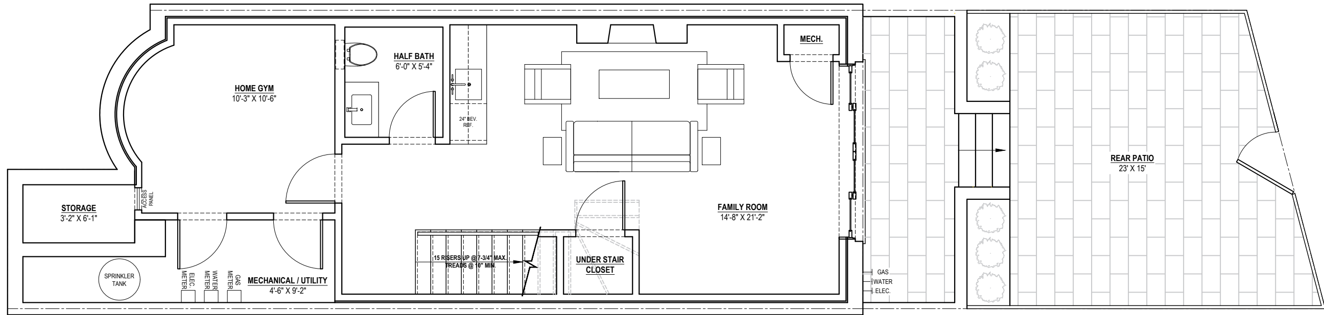
01 | PROPOSED GARDEN LEVEL PLAN 3/16" = 1'-0"
