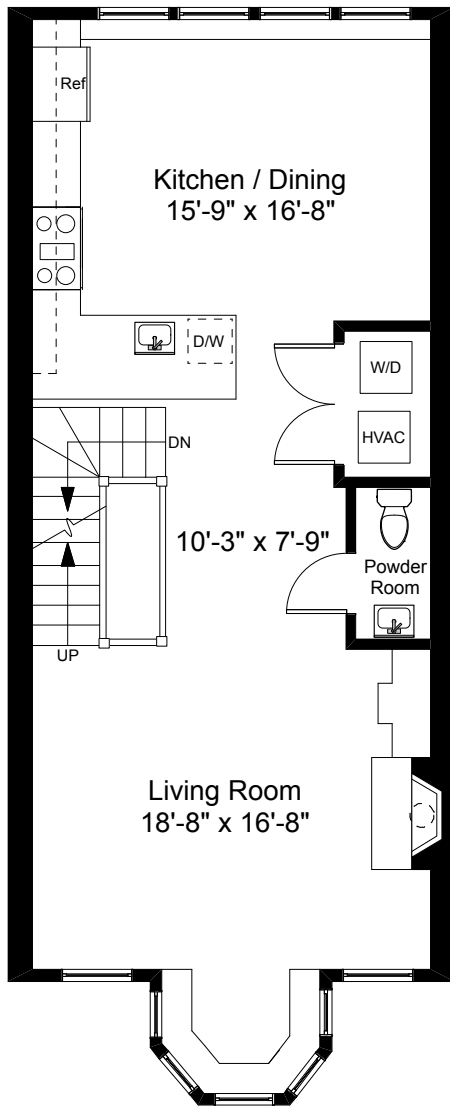
Fourth Floor Plan Ceiling Height = 8'-6"
