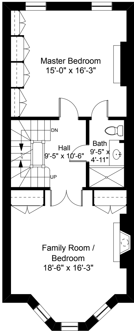
Second Floor Plan Ceiling Height = 10'-9"
