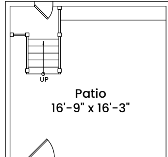
GARDEN LEVEL CEILING HEIGHT 8'-11"
